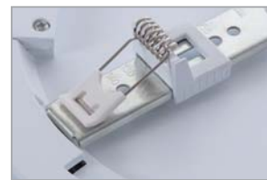
Adjustable Clip
